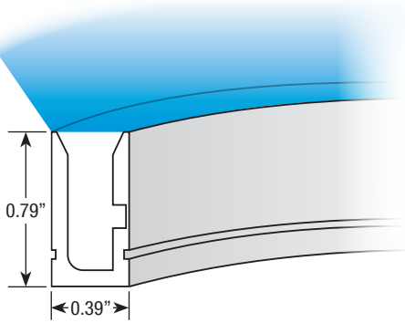
NV120S Cross Section
